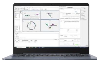
Qlucore Diagnostics
